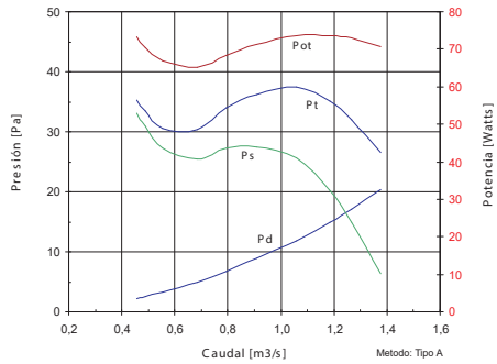
W550/8 - 3 aspas - 40°
