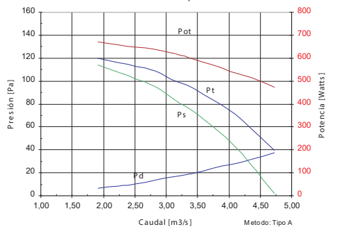
W850/8 - 4 aspas 25°
